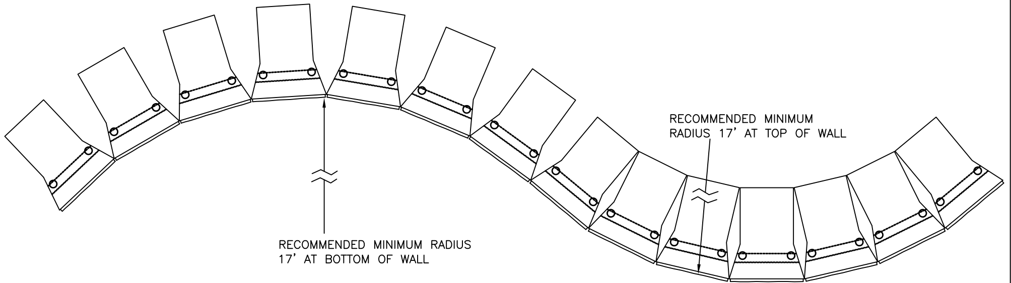
CURVE DETAIL TYPICAL CURVES SCALE: NONE
